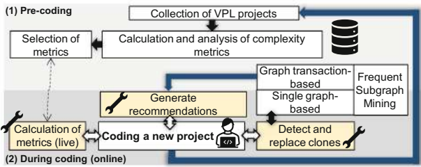
Fig. 1. Overview of the two parts to of the low-code programming assistant (adopted from [1])
